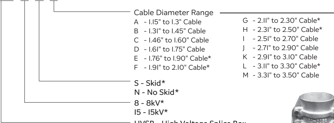
High Voltage Splice Box
