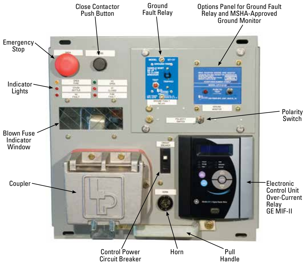
Front View
