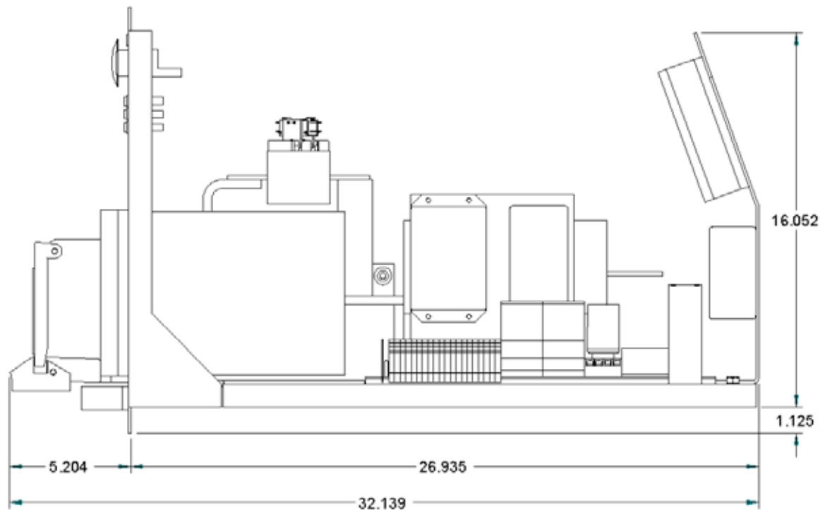
Side View
